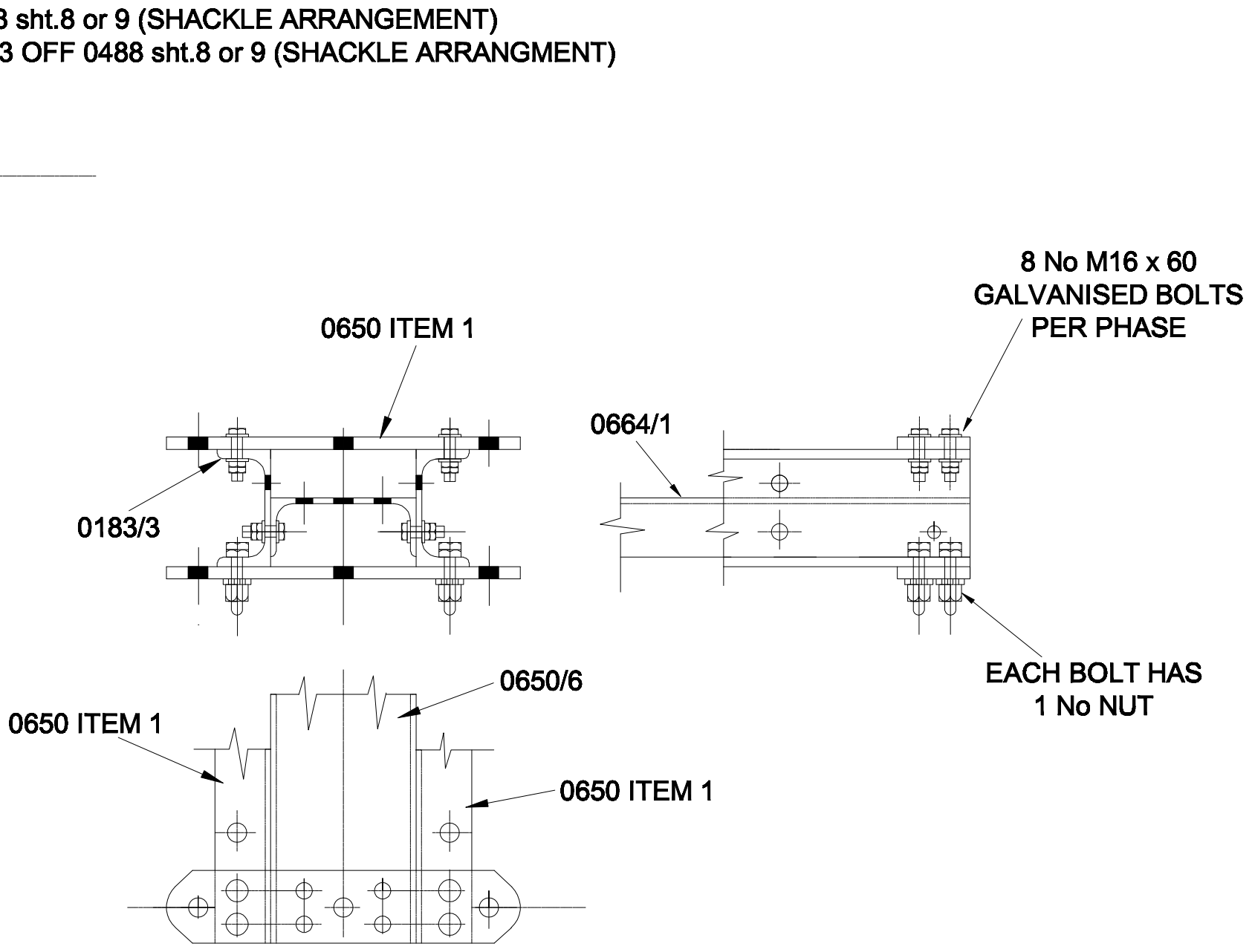
ENLARGED DETAIL ' A ' SCALE 1 : 7.5
